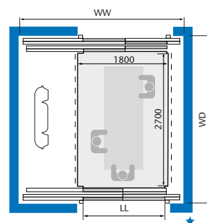
2500 kg / 33 persons Through type / side opening
