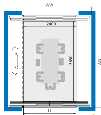
5000 kg / 67 persons Through type / center opening
