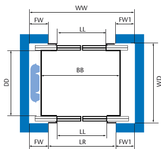
Car with front wall, door LL ≠ BB*
