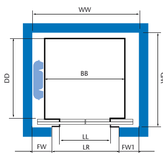
Vertical shaft arrangement for a single and a dual entrance car
